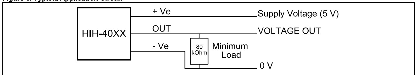
Figure 6. Typical Application Circuit
